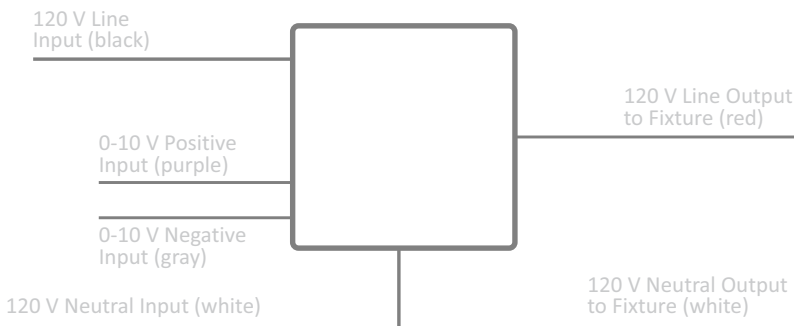
Wiring Diagram
